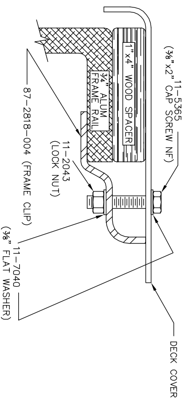
FOR ALUMINUM RAIL W/ WOOD SPACER
